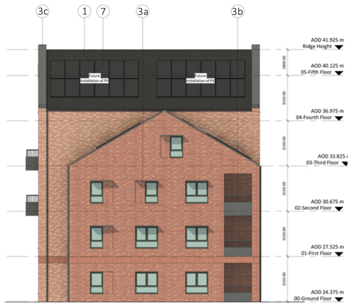
Block A - South Elevation
