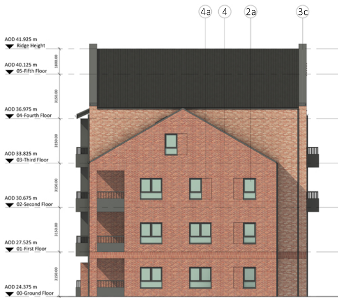
Block A - North Elevation
