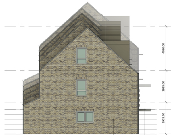
Terrace - East Elevation
