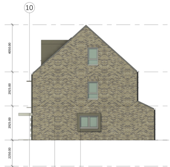
Terrace - West Elevation
