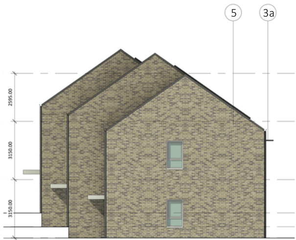
Maisonettes - West Elevation
