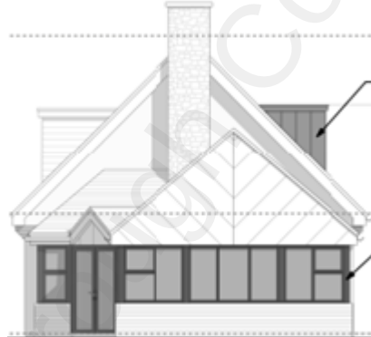
Proposed Left Side Elevation
