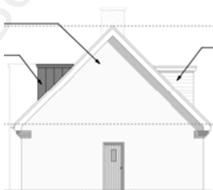
Proposed Right Side Elevation
