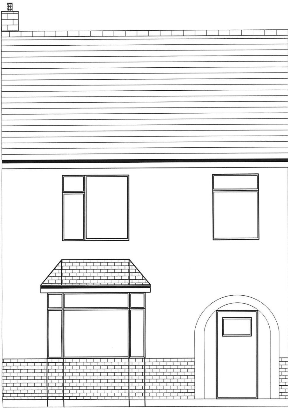
Proposed Front Elevations
