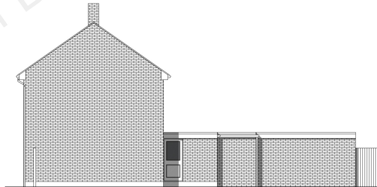
04 | 1:100 | SIDE ELEVATION
