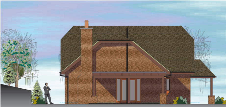
Proposed Side (South) Elevation
