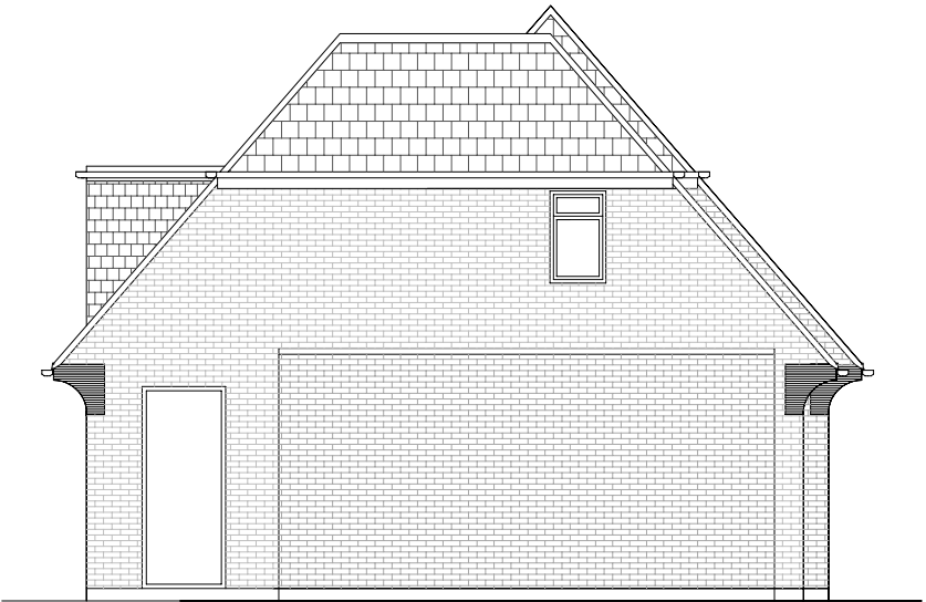
Proposed south
