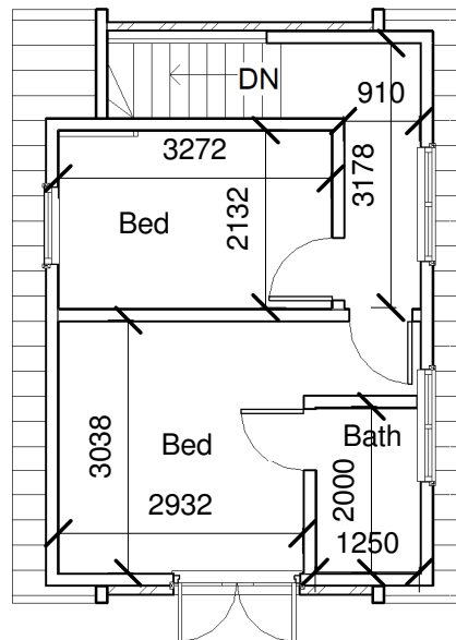
4 Proposed First Floor Plan 1 : 100
