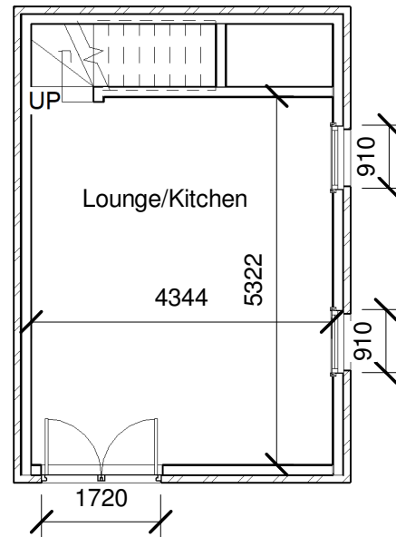
2 Proposed Ground Floor Plan 1 : 100
