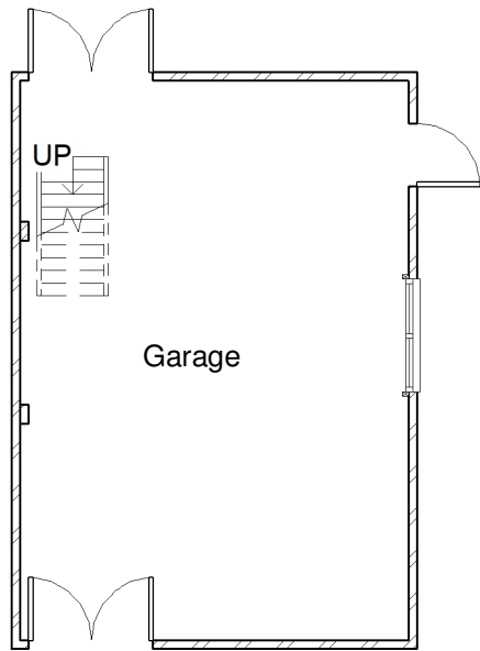
1 Existing Ground Floor Plan 1 : 100
