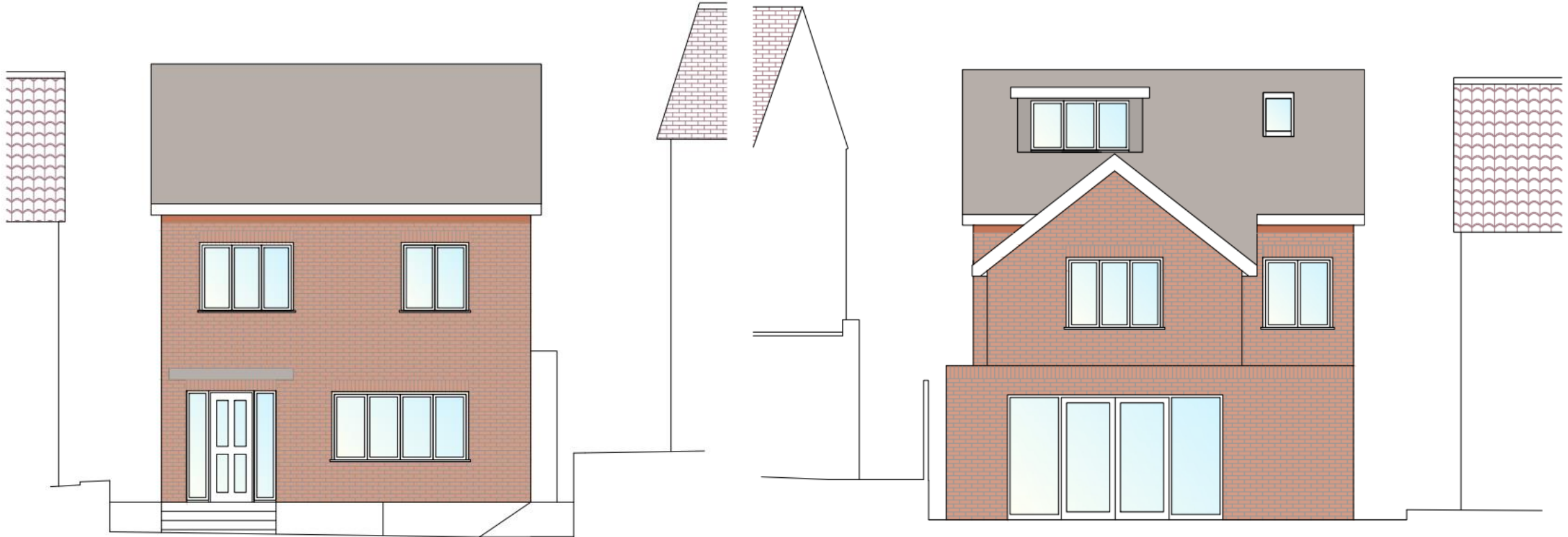
FRONT ELEVATION
