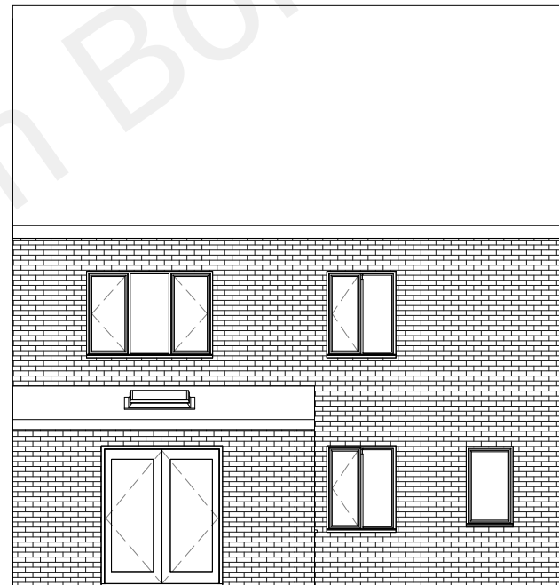
02. Rear Elevation Proposed
