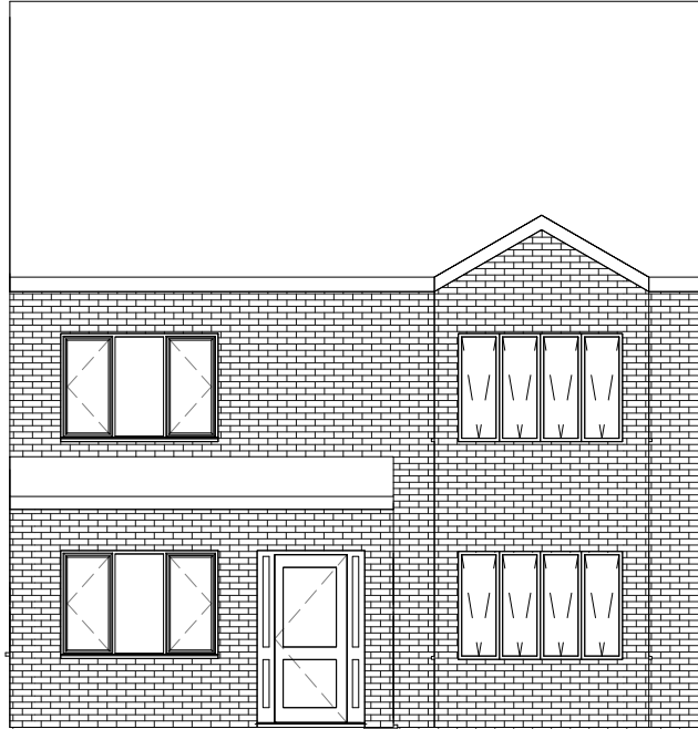
01. Front Elevation Existing
