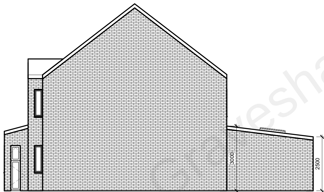
03. Right Elevation Proposed 1 : 100
