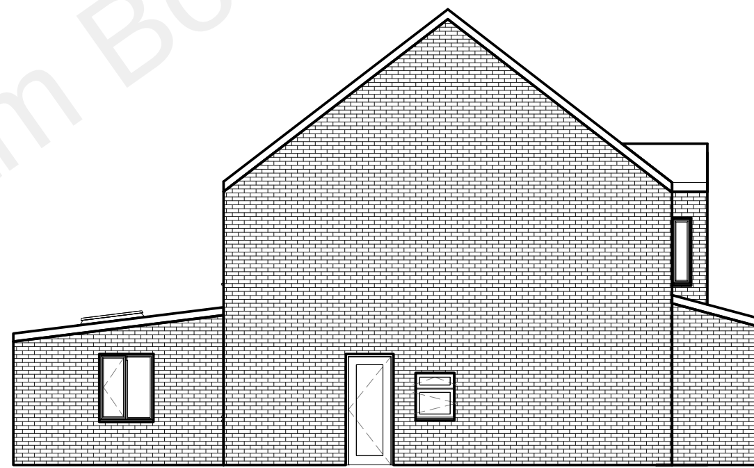
04. Left Elevation Proposed 1 : 100
