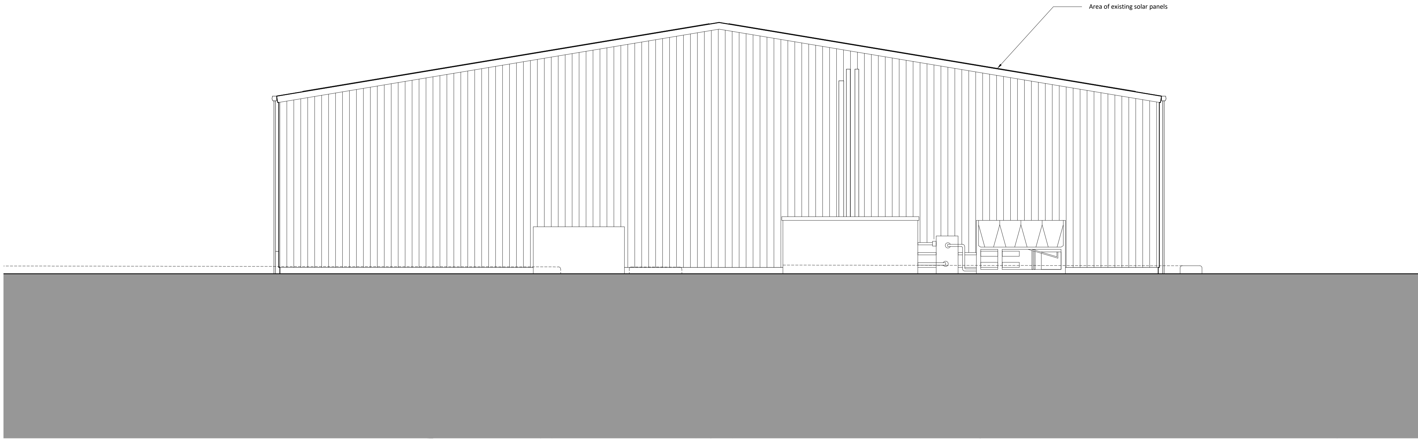
Existing Side (North-East) Elevation 1:100
