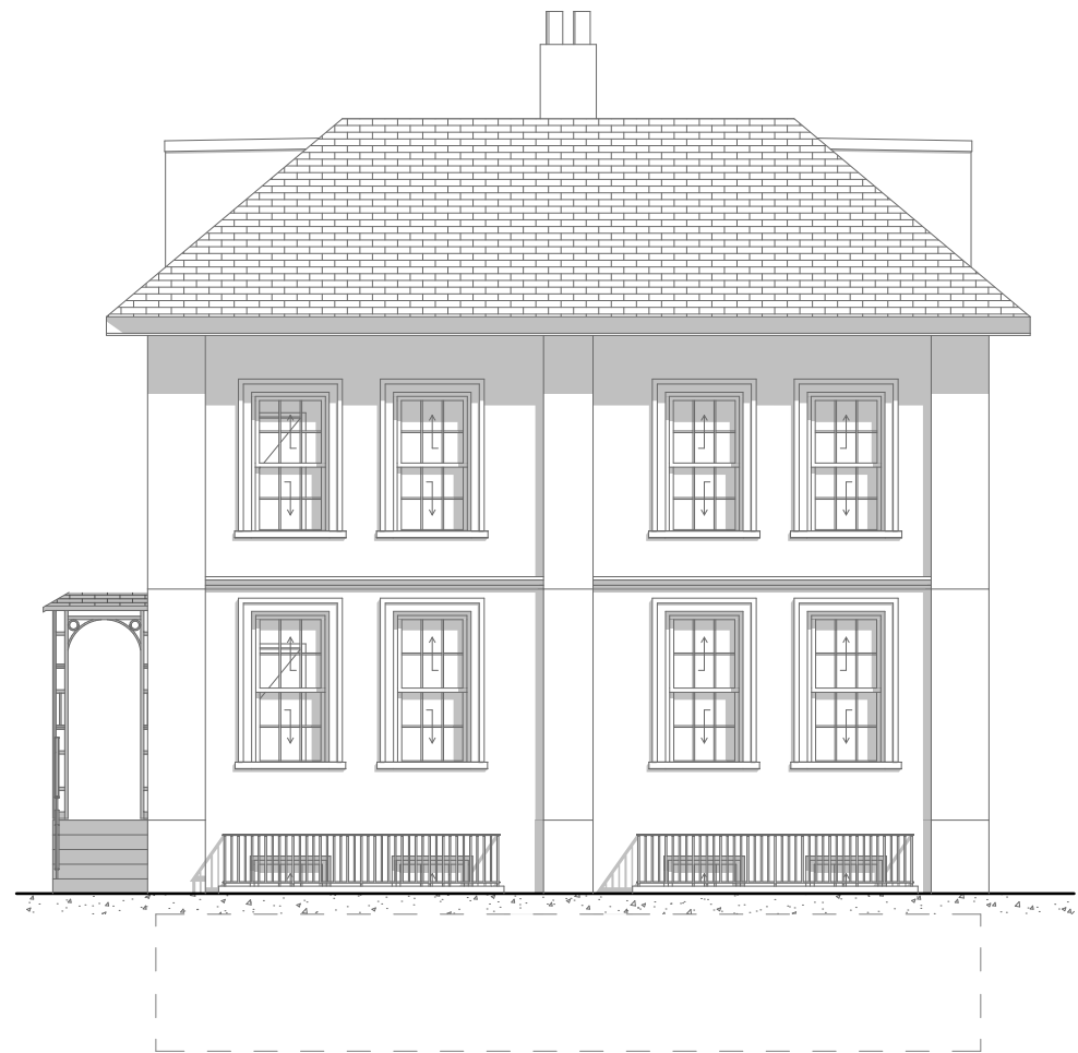
Proposed Elevations
