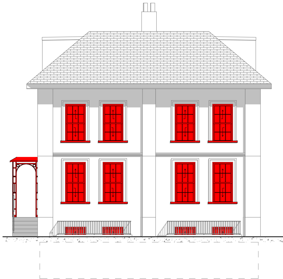
Existing Elevations
