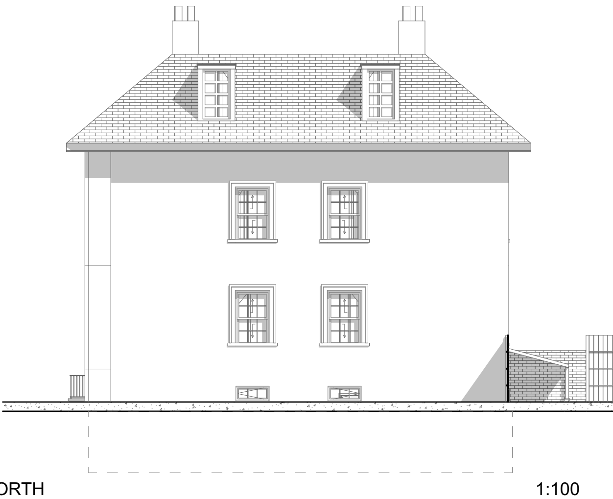
Proposed Elevations
