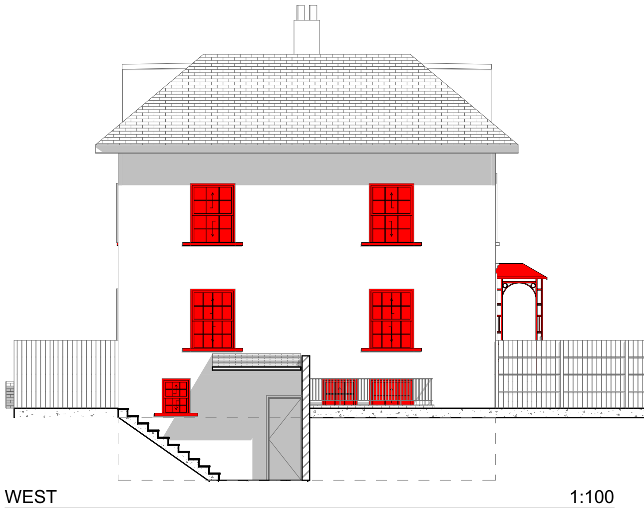
Existing Elevations
