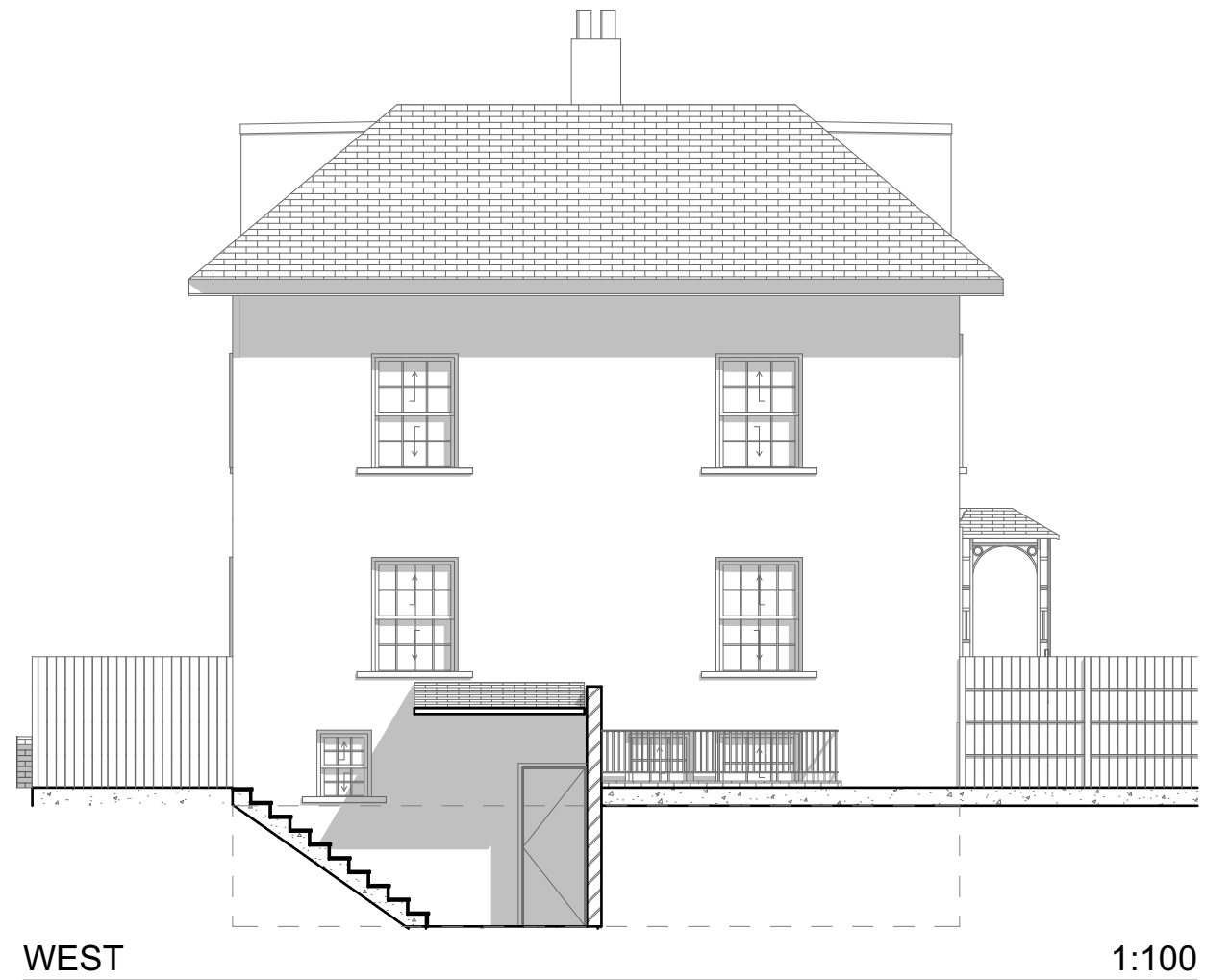
Proposed Elevations
