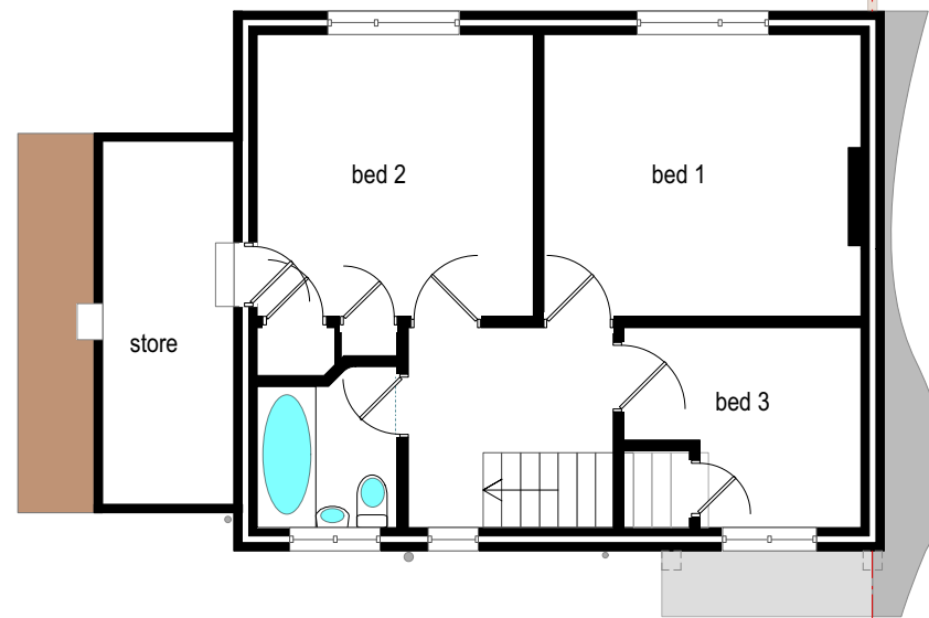
first floor 51 m 2 including attic store
