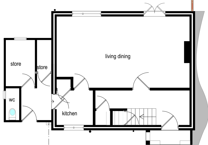
ground floor 55 m 2 including stores
