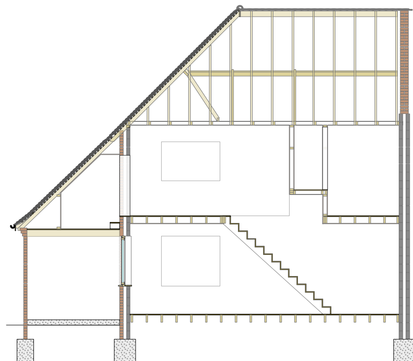
section south - north through staircase
