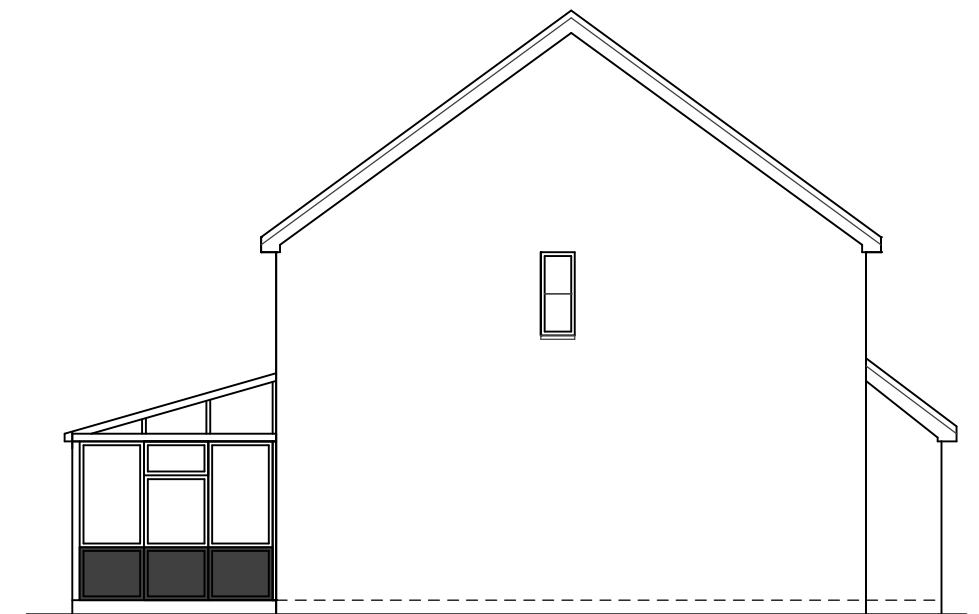
left (southeast) elevation
