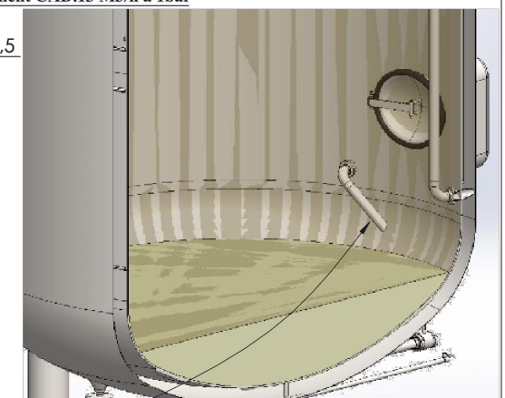
DETAIL ADJUSTABLE INTERNAL PIPE WITH EMPTY TANK
