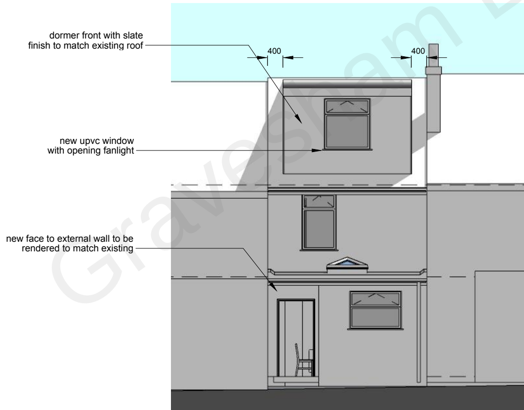
d garden / west elevation 004 scale: 1:100
