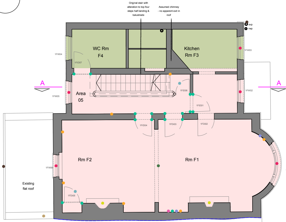
First Floor Heritage and Phasing Plan
