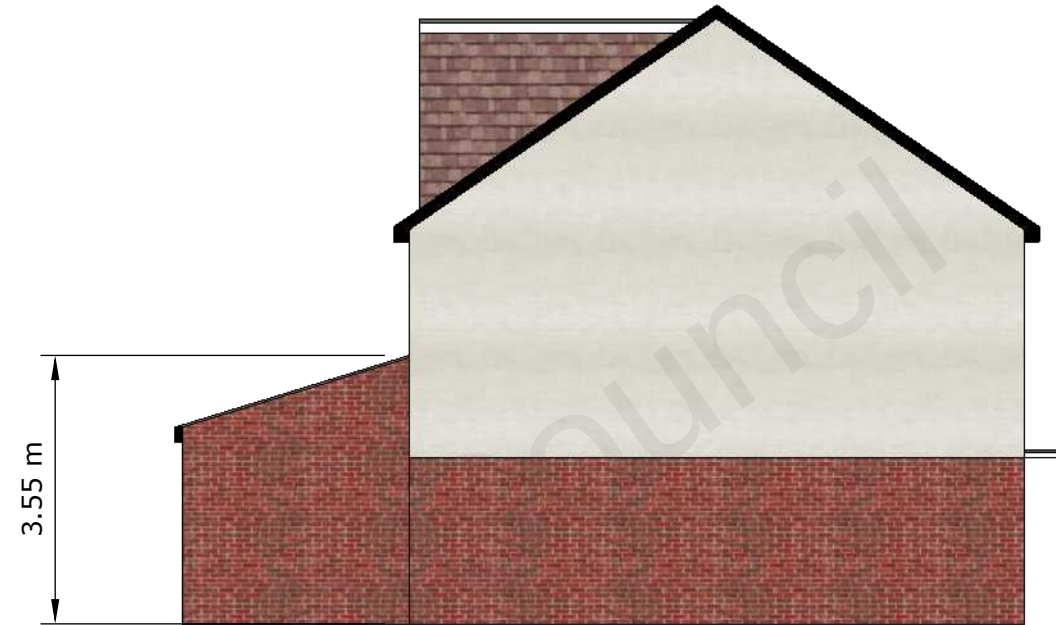
West Elevation
