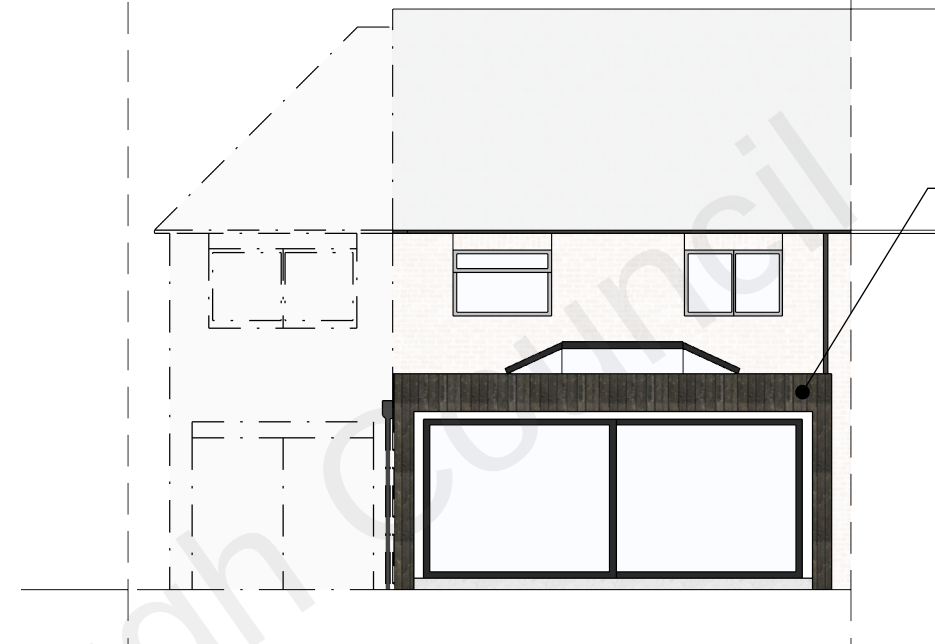
Rear Elevation
