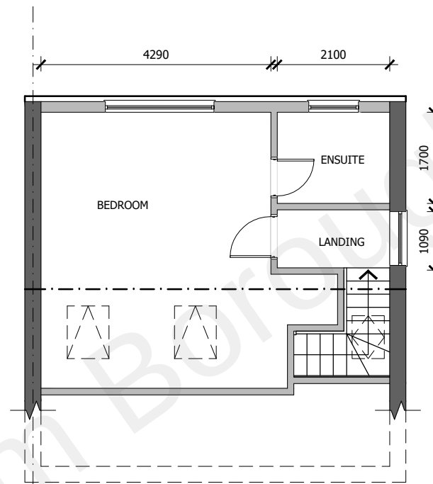
PROPOSED LOFT PLAN
