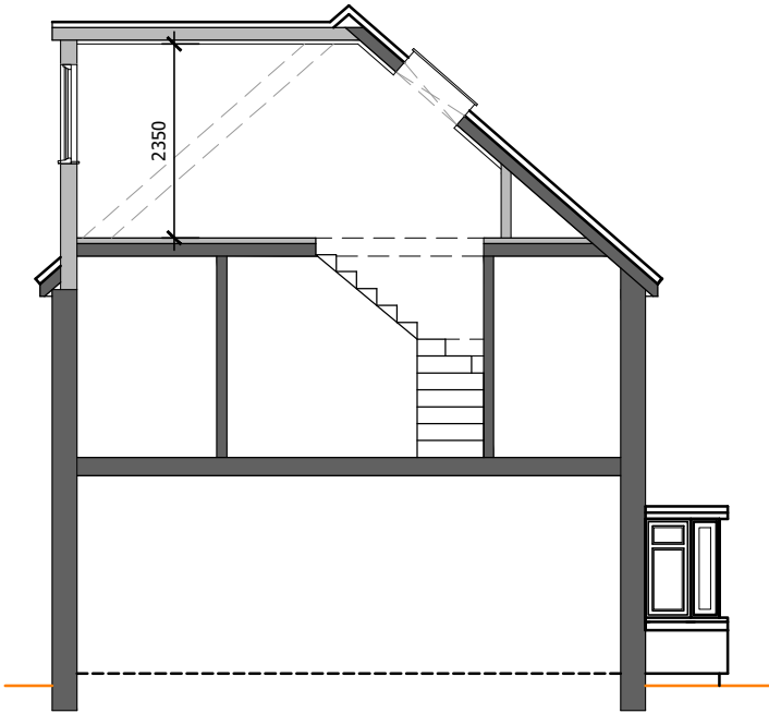
PROPOSED SECTION
