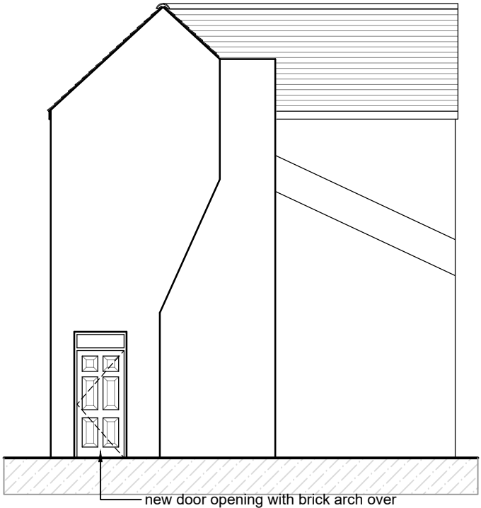
SIDE ELEVATION (1:100)
