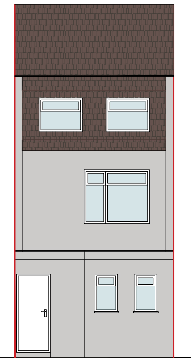
Rear Elevation
