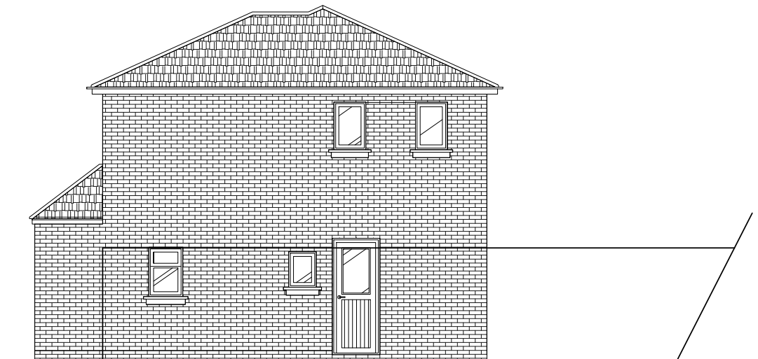
EXISTING RIGHT ELEVATION
