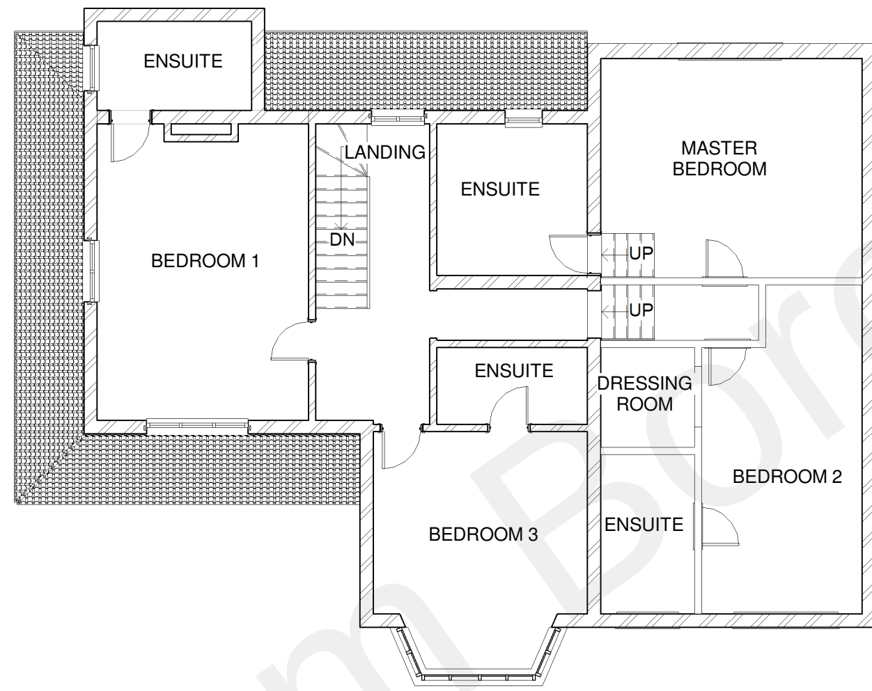
06 FIRST FLOOR 1 : 100
