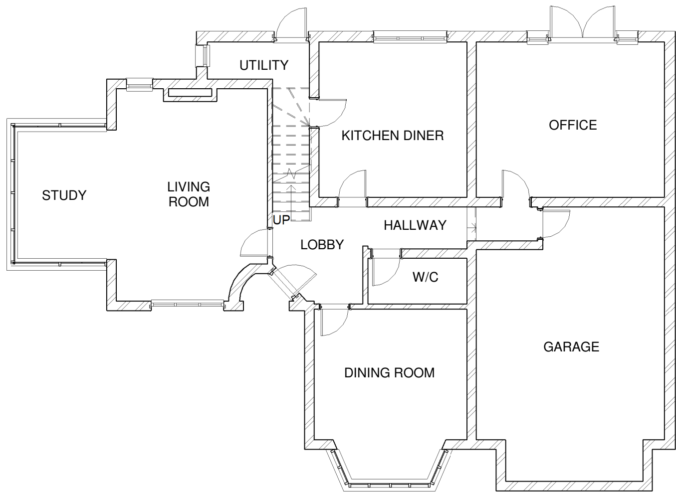
05 GROUND FLOOR 1 : 100
