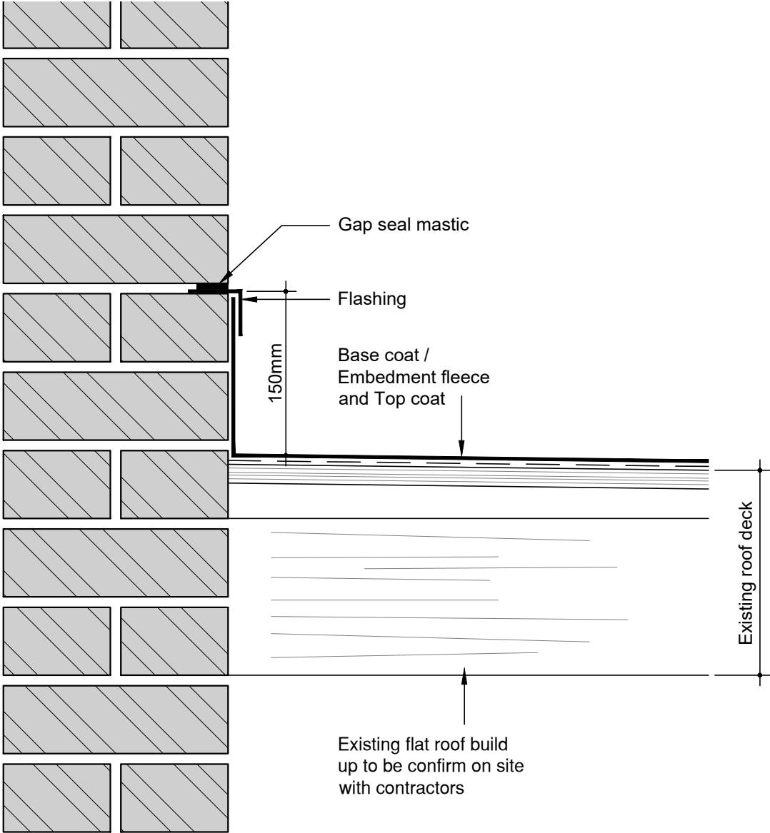
TYPICAL FLAT ROOF ABUTMENT DETAIL UNINSULATED SYSTEM
