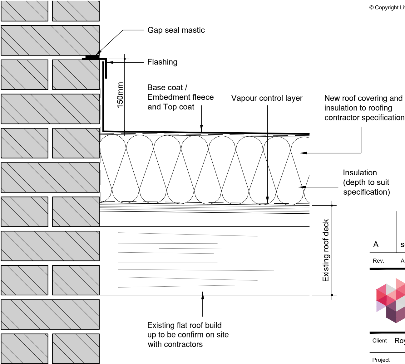
TYPICAL FLAT ROOF ABUTMENT DETAIL INSULATED SYSTEM
