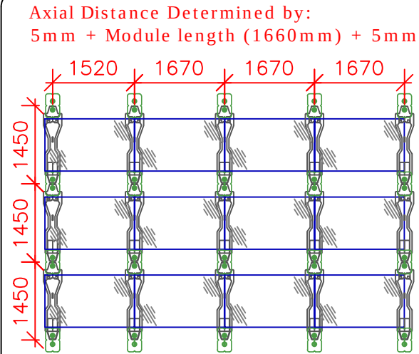
Grid Arrangement 1:100
