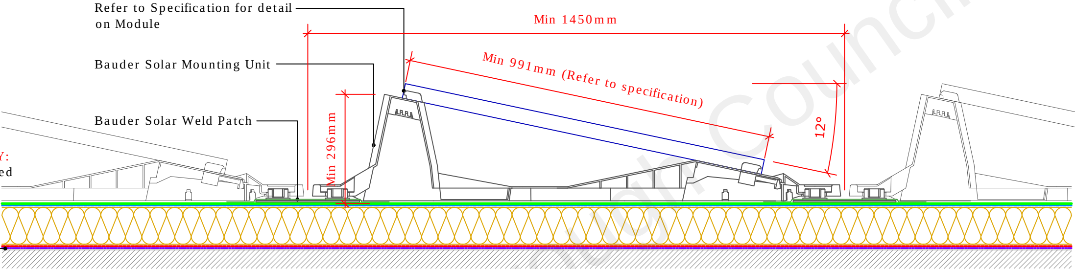
Solar Module Section - Scale 1:10
