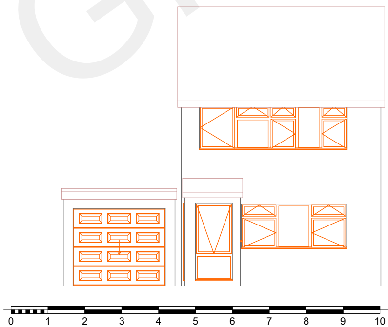
4 South Elevation Existing 1:100
