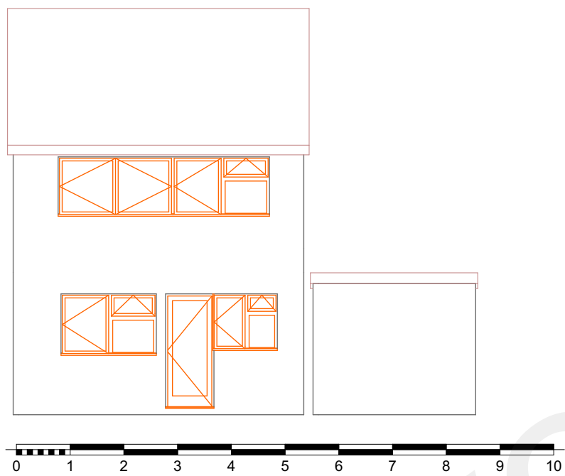
3 North Elevation Existing 1:100
