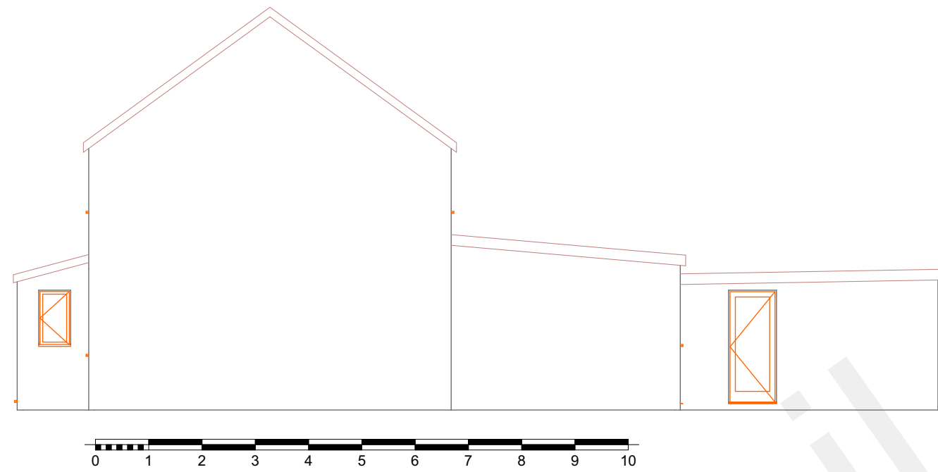
5 East Elevation Proposed 1:100
