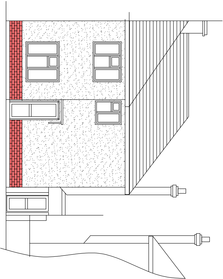
Front Elevation
