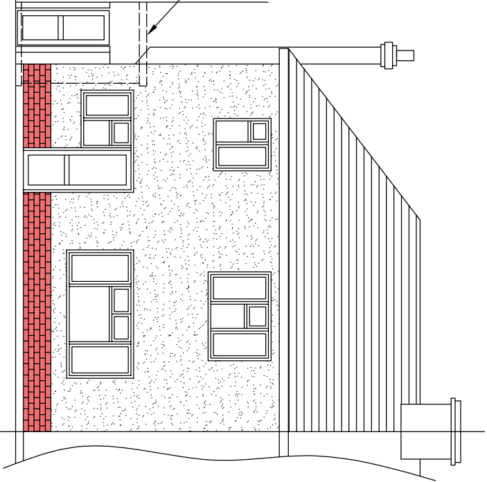
Rear Elevation
