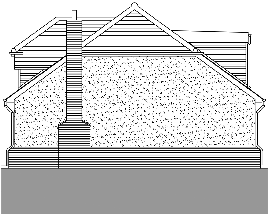
Proposed Side (South) Elevation 1100
