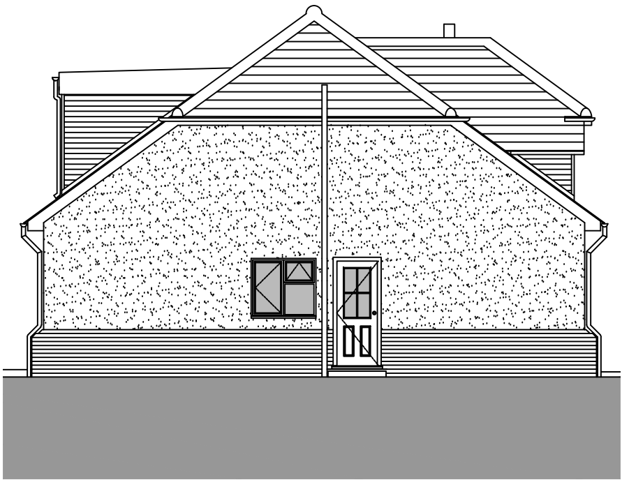
Proposed Side (North) Elevation 1100
