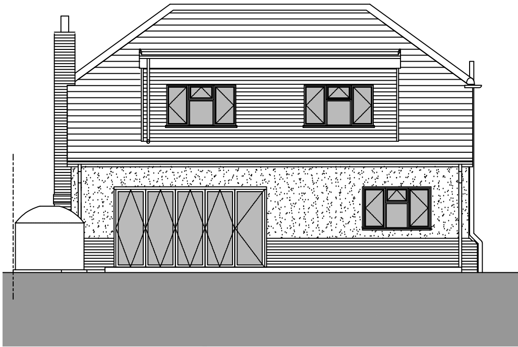
Proposed Rear (East) Elevation 1100
