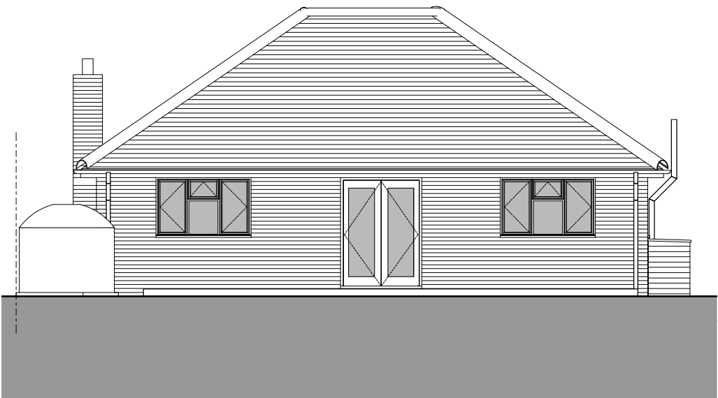
Existing Rear (East) Elevation 1100
