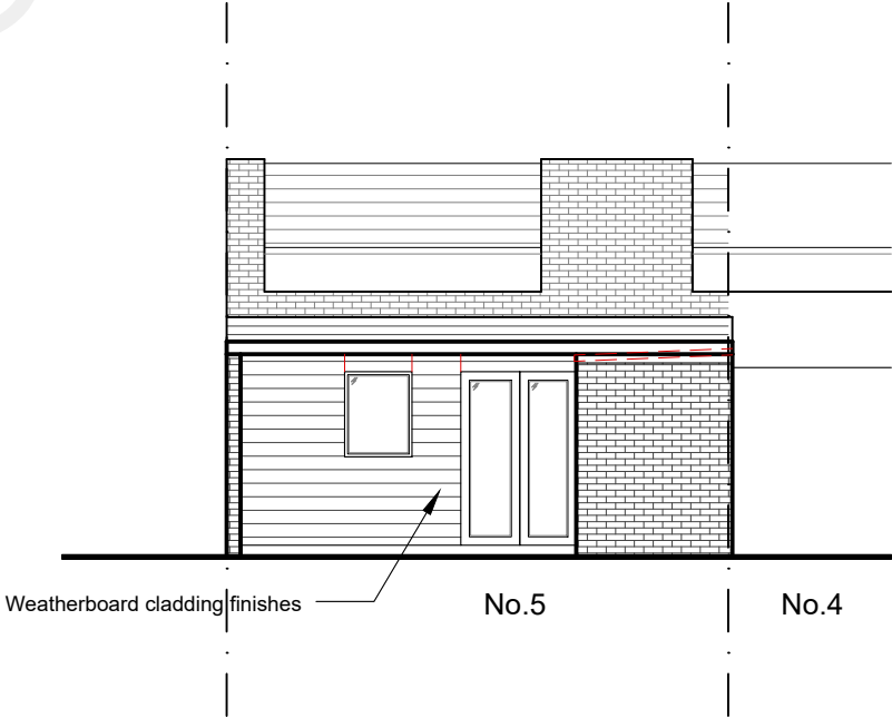
PROPOSED REAR (NORTH) ELEVATION
