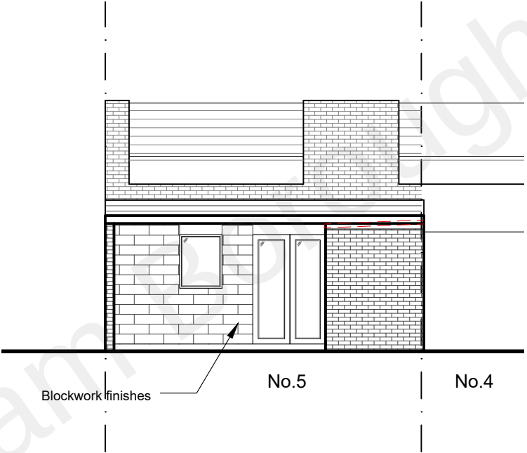
CURRENT REAR (NORTH) ELEVATION
