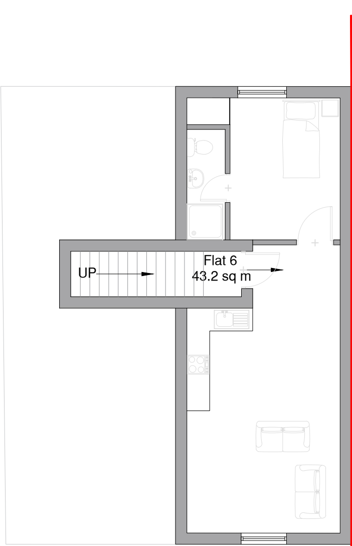
THIRD FLOOR
