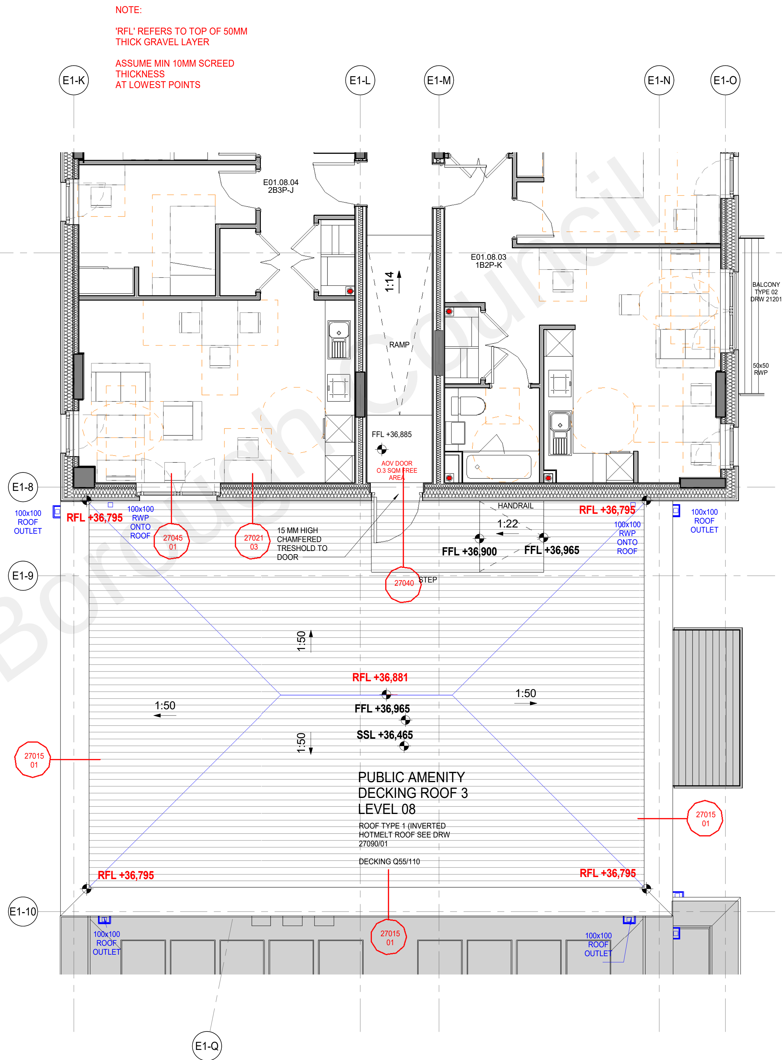
2 E01 FLAT ROOF LEVEL 08 SOUTH 2/2 1:50
