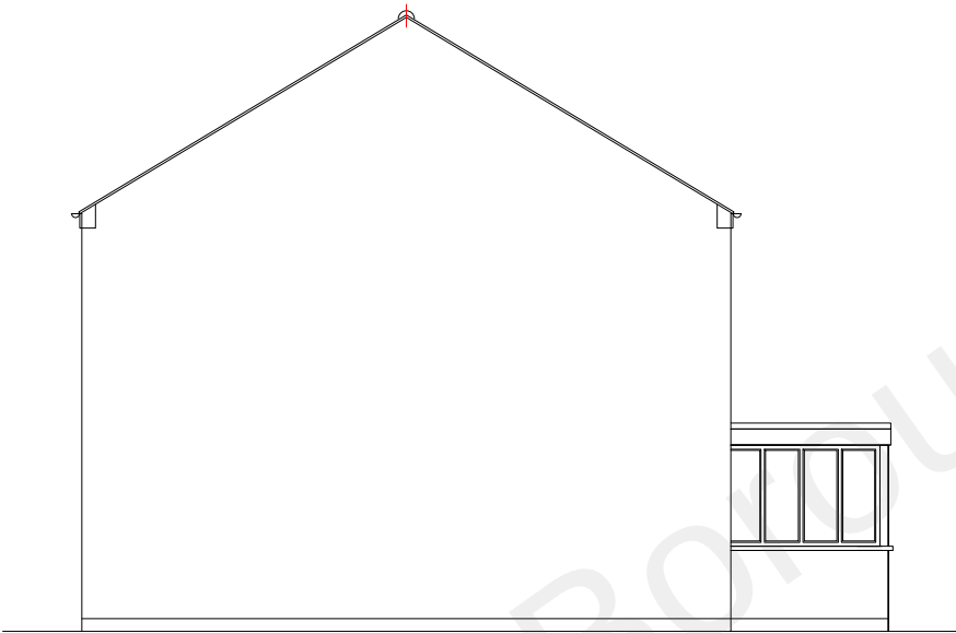
WEST ELEVATION
