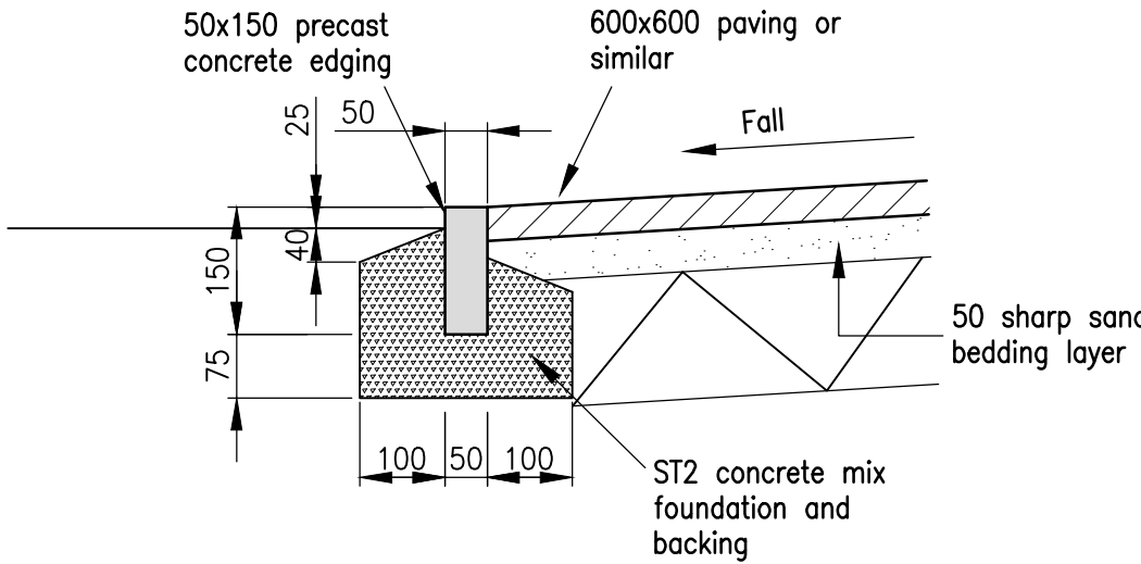
Precast Concrete Kerb Detail Scale 1:10
