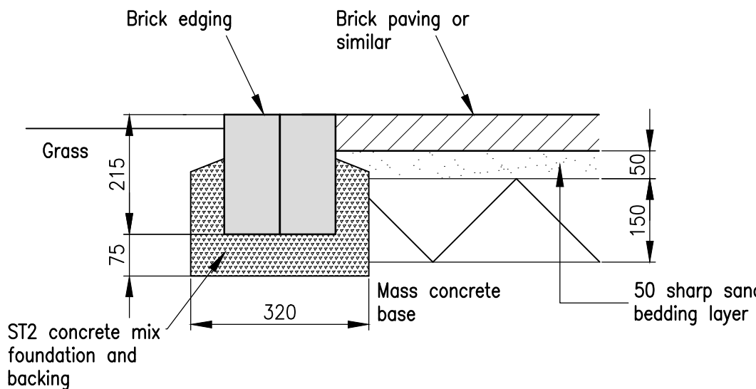
Brick Kerb Detail Scale 1:10
