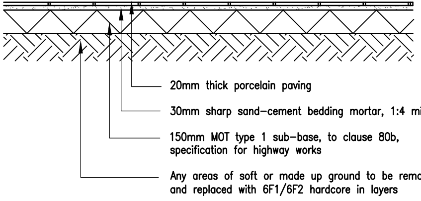
Porcelain Paving Construction Detail Scale 1:20
