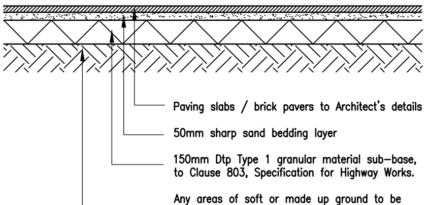
Paving / Brick Pavers Construction Detail Scale 1:20
