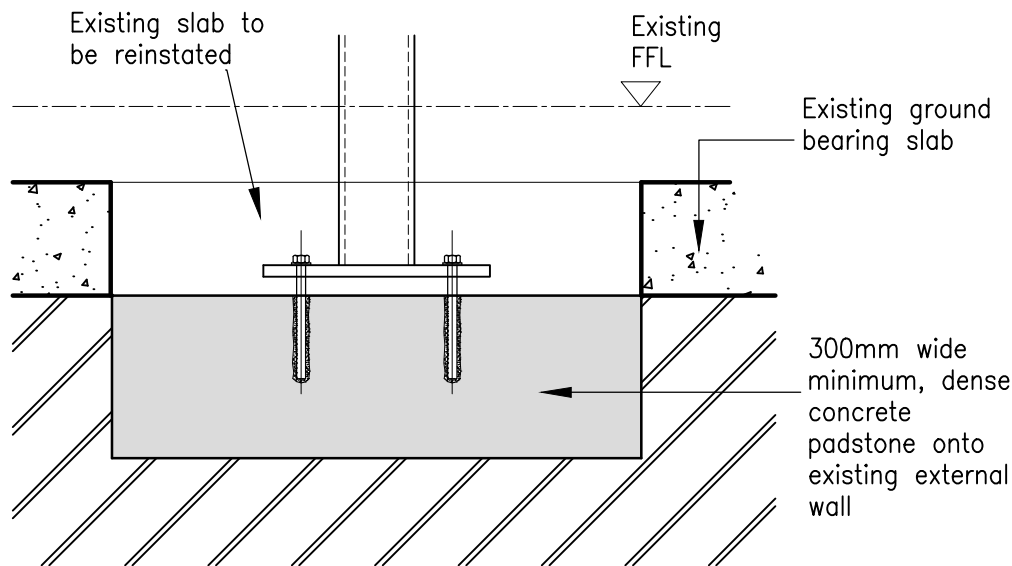
Typical Column Padstone Detail
