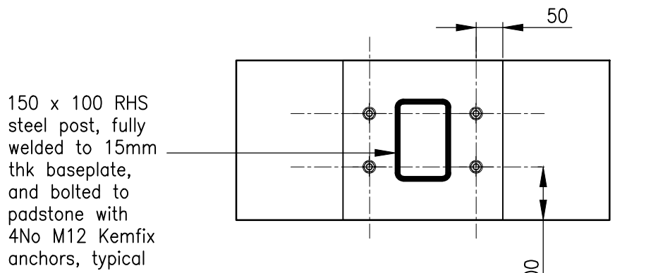
Column/Padstone on Plan
