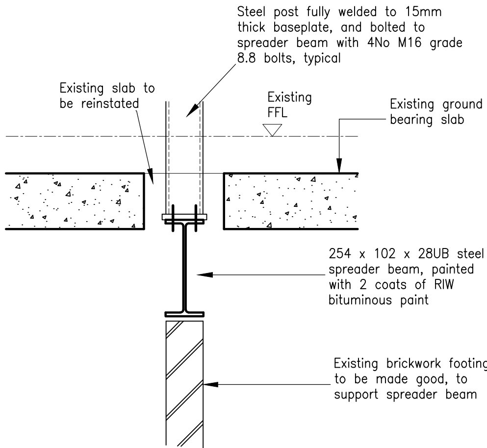
Section through Spreader Beam
