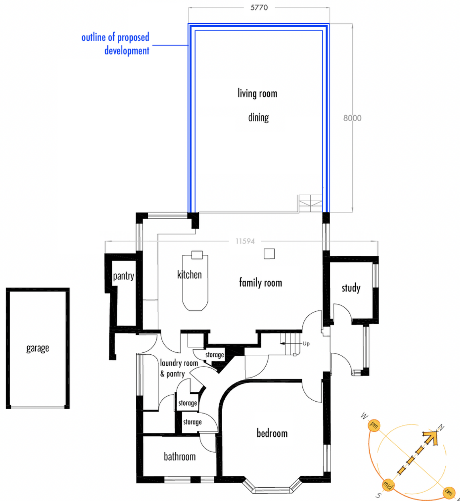
Ground Floor | Proposed
