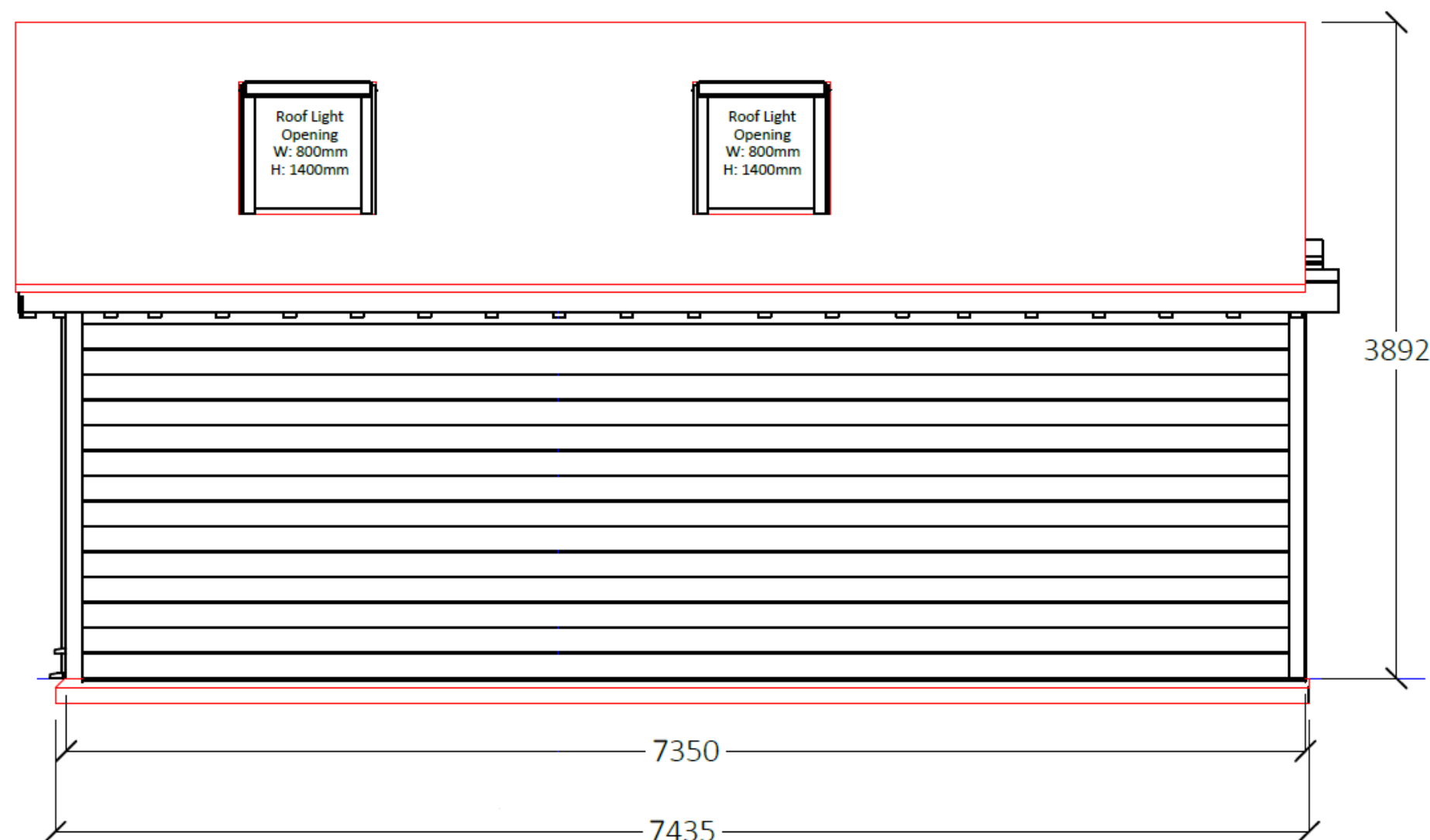
North Elevation
