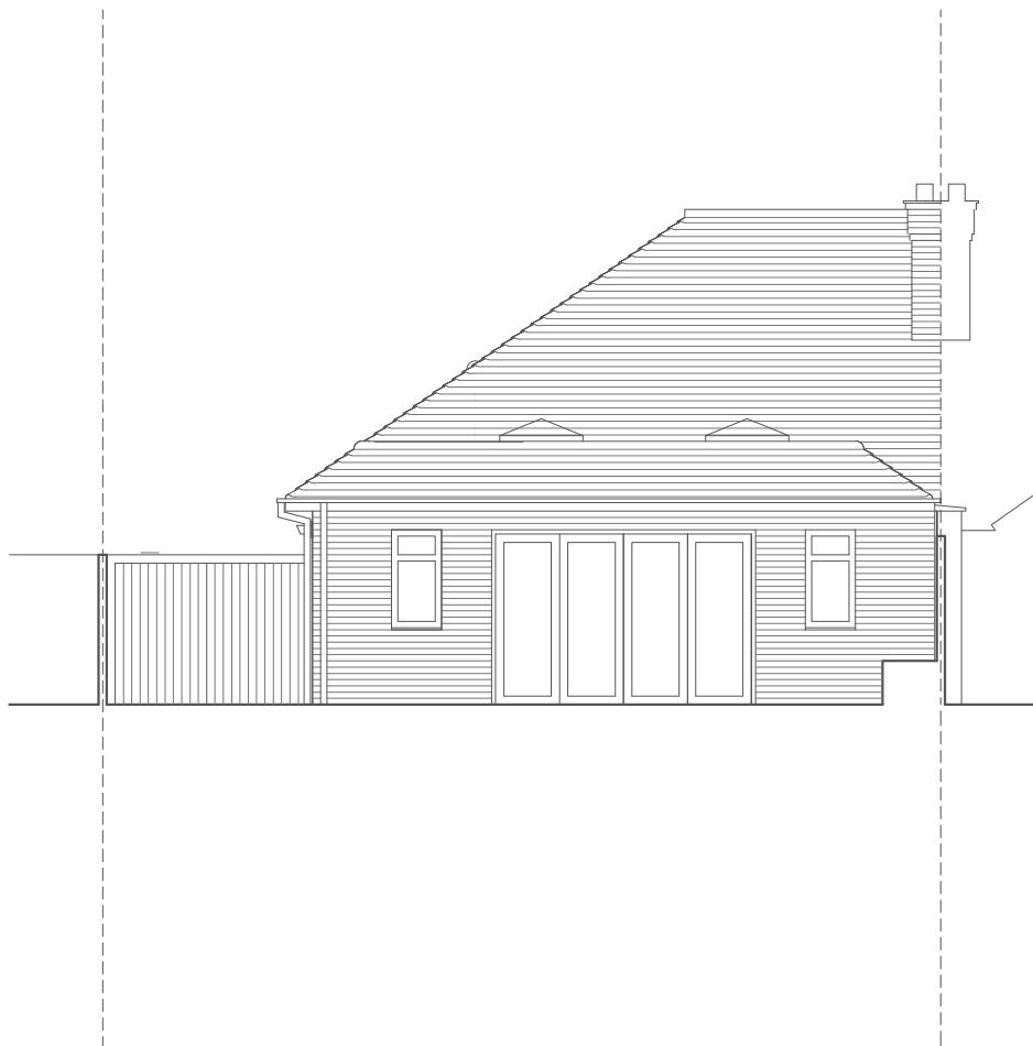
North East Elevation
