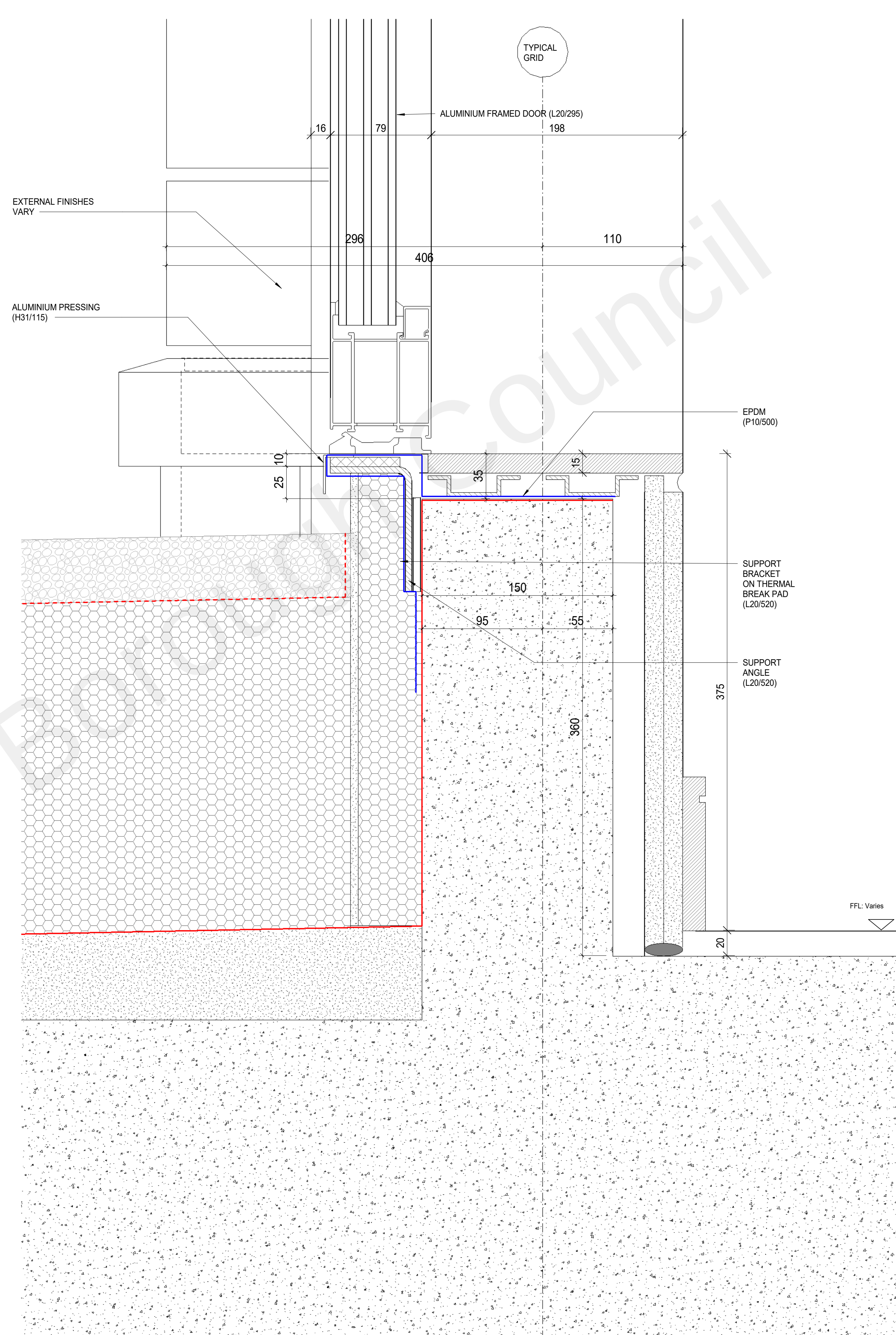
2 SITEWIDE SIDE HUNG DOOR TERRACE THRESHOLD
