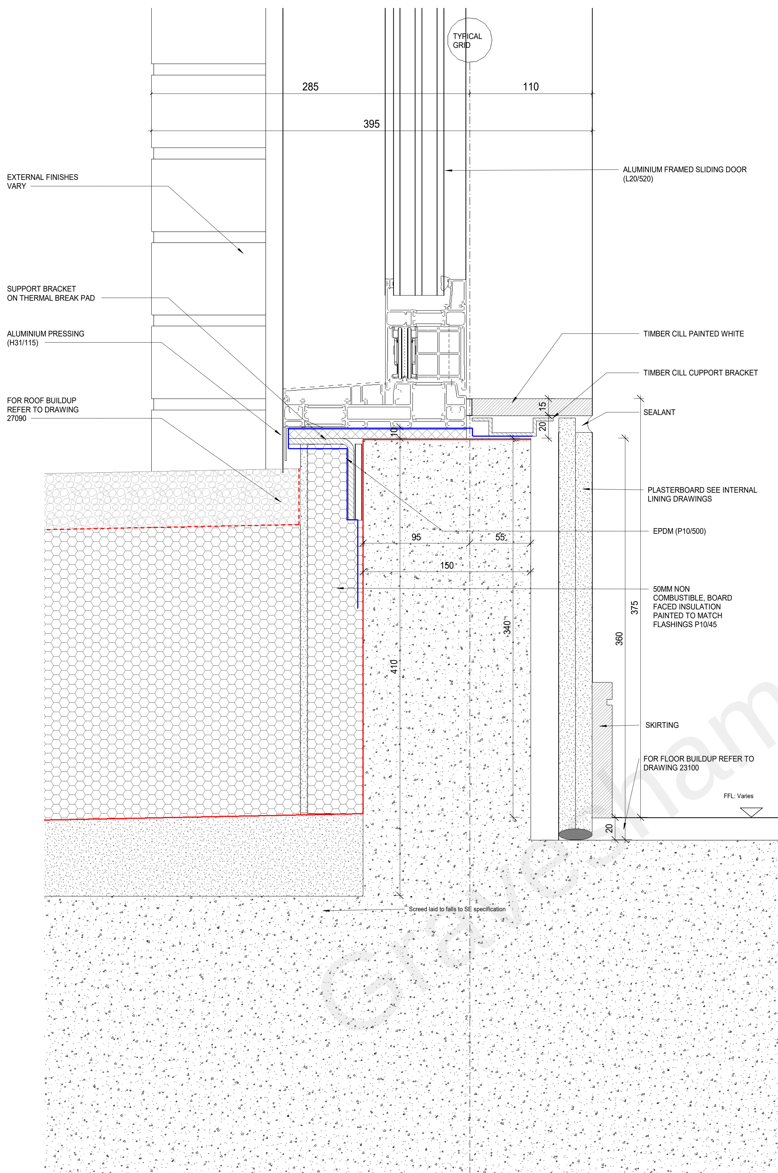
1 SITEWIDE SLIDING DOOR TERRACE THRESHOLD
