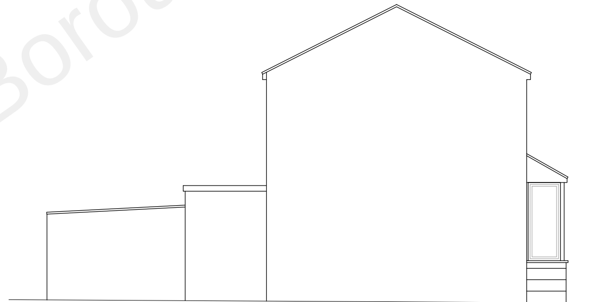
Side Elevation 1:100
