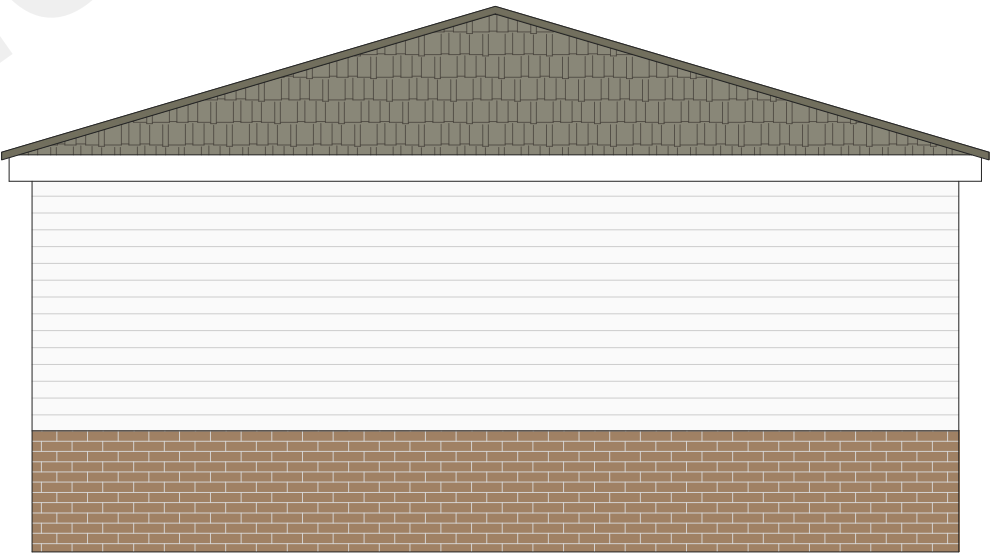
South Elevation
