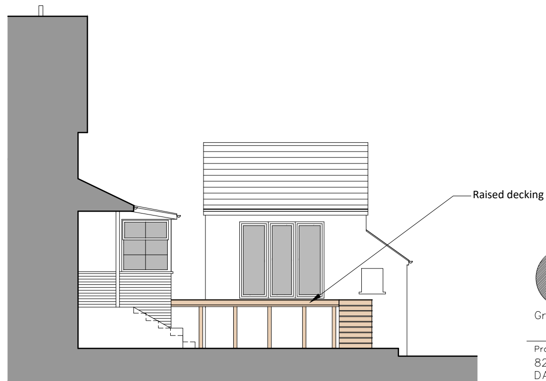
Existing Raised Decking Side (West) Elevation 1:100
