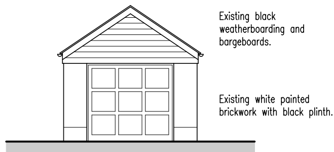
Front Elevation West
