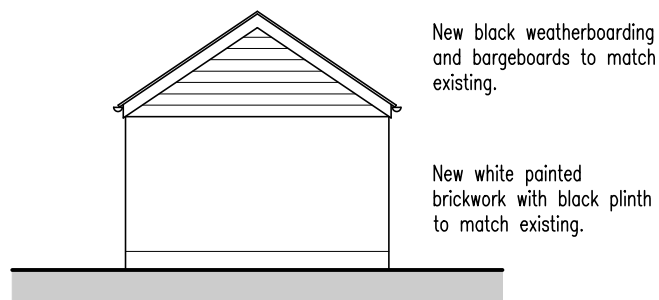
Rear Elevation East
