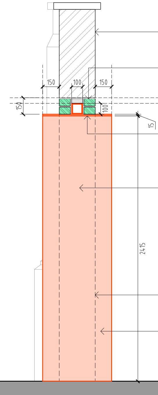
Spine Wall Opening Section
