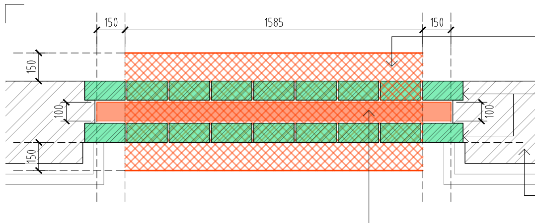
Spine Wall Opening Plan (head of opening)
