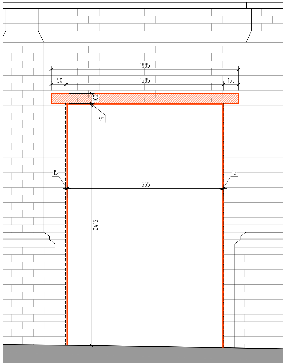
Spine Wall Opening Elevation
