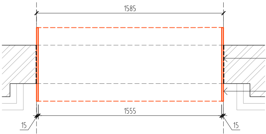
Spine Wall Opening Plan (middle of opening)
